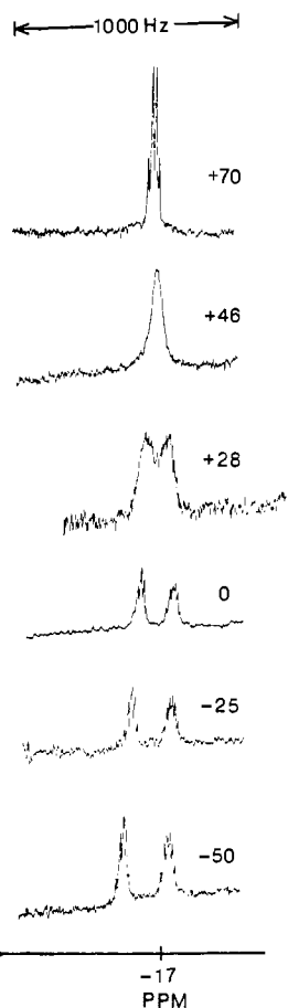
Figure 3. Temperature-dependent 220-MHz ^1\text{H} NMR for \text{RhCl}(\text{P}(p\text{-tolyl})_3)_2\text{py}(\text{H})_2 , relative to \text{Me}_4\text{Si} .
