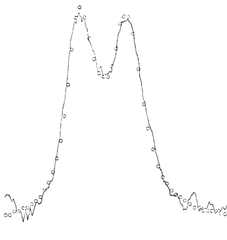
Figure 4. 220-MHz spectrum of \text{RhCl}(\text{P}(4\text{-tolyl})_3)_2(\text{H})_2 at 27^\circ\text{C} showing experimental (—) and calculated (○) values based on an exchange reaction that assumes first-order dissociation of pyridine.
