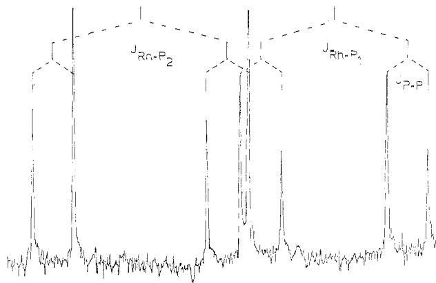
Figure 1. ^{31}\text{P} NMR spectrum of \text{RhCl}(\text{P}(4\text{-tolyl})_3)_2\text{py} .
