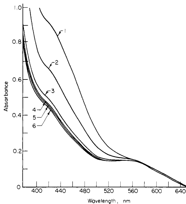
Figure 5. UV spectrum of a toluene solution of 2.98 \times 10^{-3}\text{ M} [\text{RhCl}(\text{P}(4\text{-tolyl})_3)_2]_2 and 5.79 \times 10^{-2}\text{ M} THTP at 10.0^\circ\text{C} in equilibrium with various pressures of \text{H}_2 : 1, P_{\text{H}_2} = 0.00 atm; 2, P_{\text{H}_2} = 0.015 atm; 3, P_{\text{H}_2} = 0.102 atm; 4, P_{\text{H}_2} = 0.217 atm; 5, P_{\text{H}_2} = 0.371 atm; 6, P_{\text{H}_2} = 0.967 atm.
